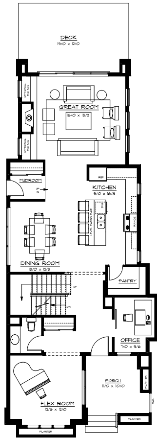
MAIN LEVEL 1255 SQ.FT
