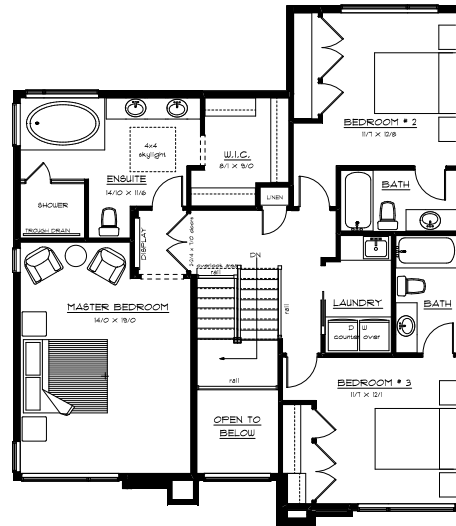
UPPER LEVEL 1279 SQ.FT
