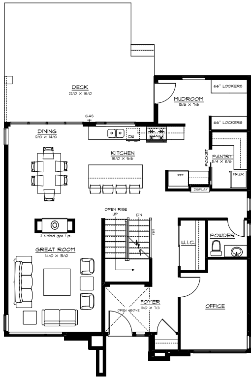
MAIN LEVEL 1323 SQ.FT
