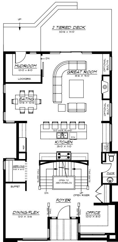
MAIN LEVEL 1550 SQ.FT
